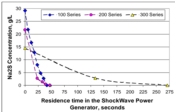
Figure 10: Sulfide concentrations vs. total residence time in the controlled cavitation device for the 100, 200, and 300 series runs.
