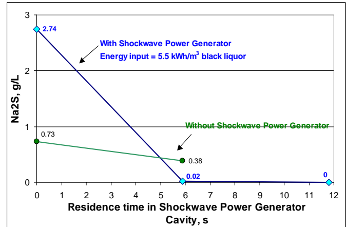
Figure 9: Sodium sulfide concentration in black liquor vs. residence time in the controlled cavitation unit cavity at nearly complete sulfide oxidation.
