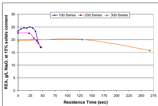
Figure 13: Residual effective alkali concentrations in black liquor vs. residence time for the oxidation run series.
