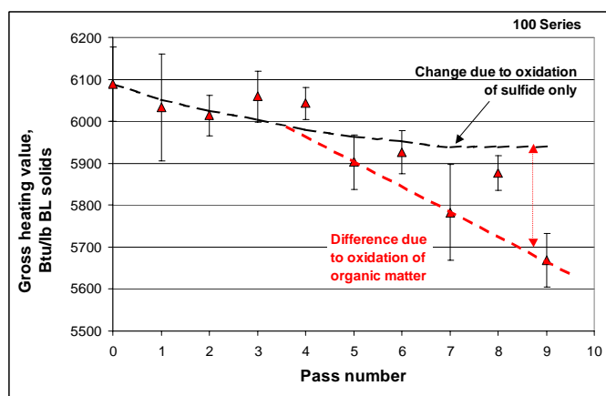
Figure 12: Na_2S concentration and gross heating value per pass for the 100 series runs.
