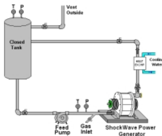
Figure 4: Experimental setup for foam control when oxidizing black liquor with air.
